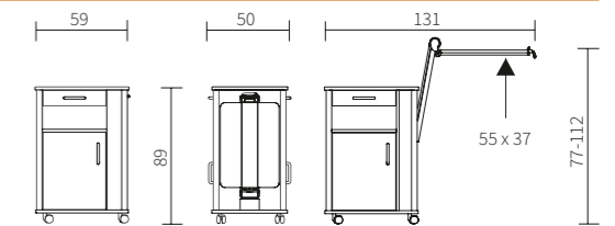
▲ The height-adjustable overbed table is easy to tilt.
